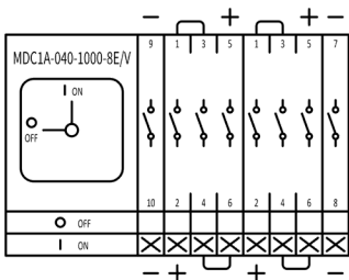
MDC1A-040-1000-12 V IEC UL
